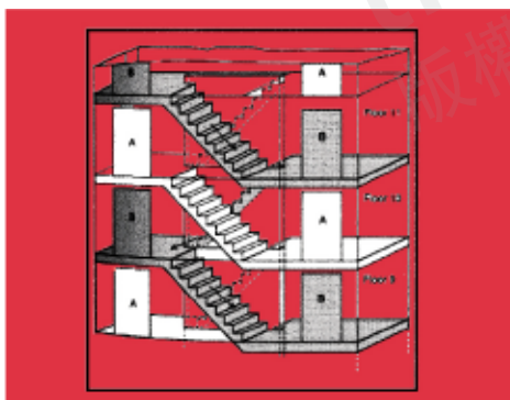
鉸剪梯 Scissors staircases
